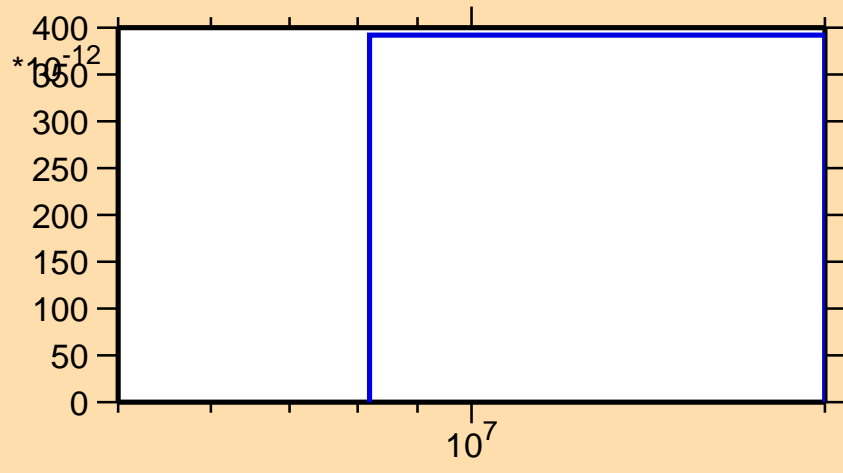
\sigma vs. E for ^{119}\text{In}(n,nt)
