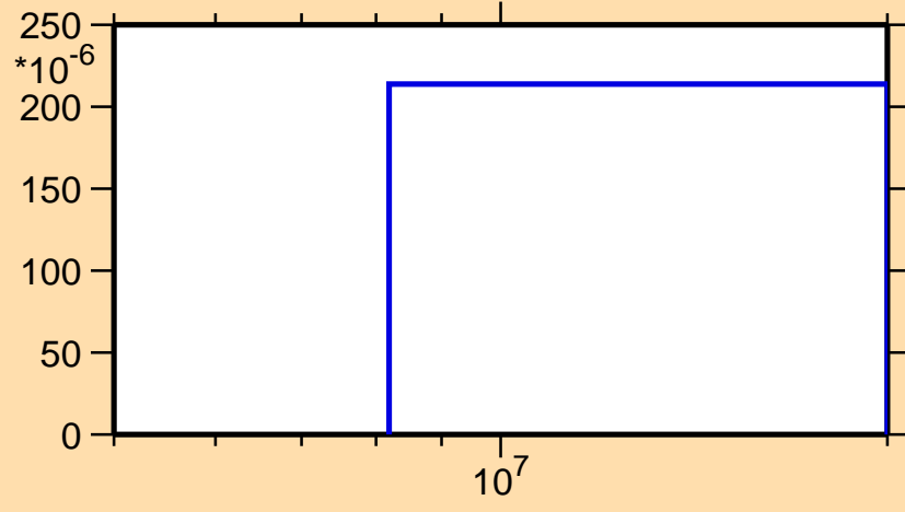
\sigma vs. E for ^{119}\text{In}(n,np)
