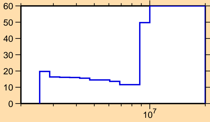
\Delta\sigma/\sigma vs. E for ^{119}\text{In}(n,n\text{cont.})
