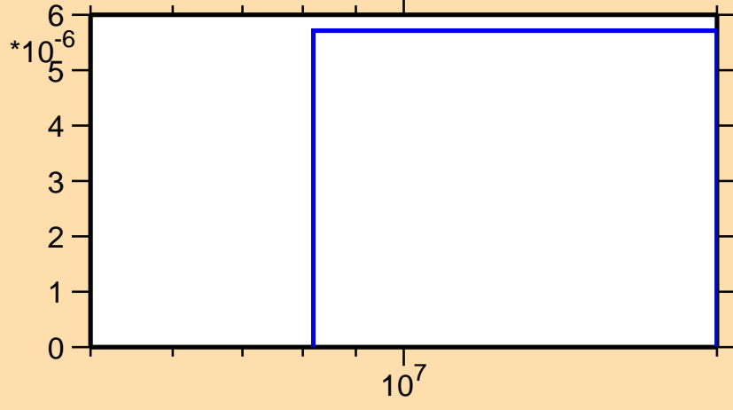
\sigma vs. E for ^{119}\text{In}(n,\alpha)
