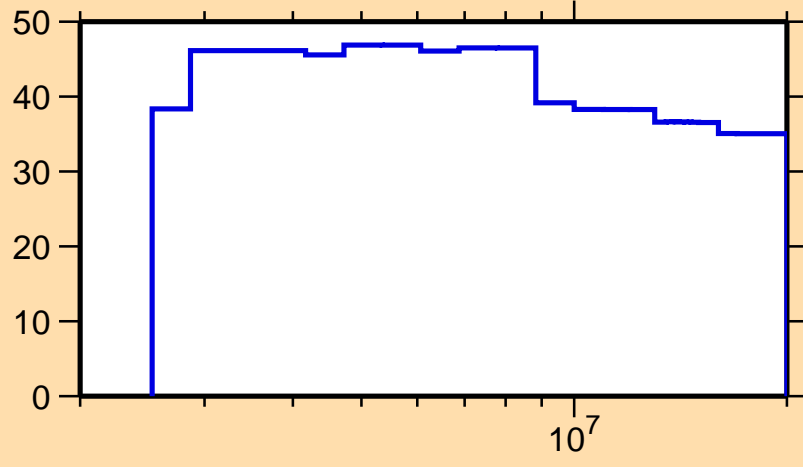
\Delta\sigma/\sigma vs. E for ^{120}\text{In}(n,p)
