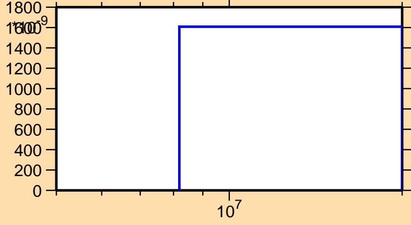
\sigma vs. E for ^{120}\text{In}(n,n\alpha)
