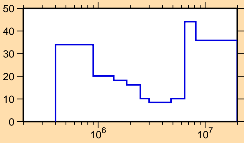
\Delta\sigma/\sigma vs. E for ^{120}\text{In}(n,n\text{cont.})
