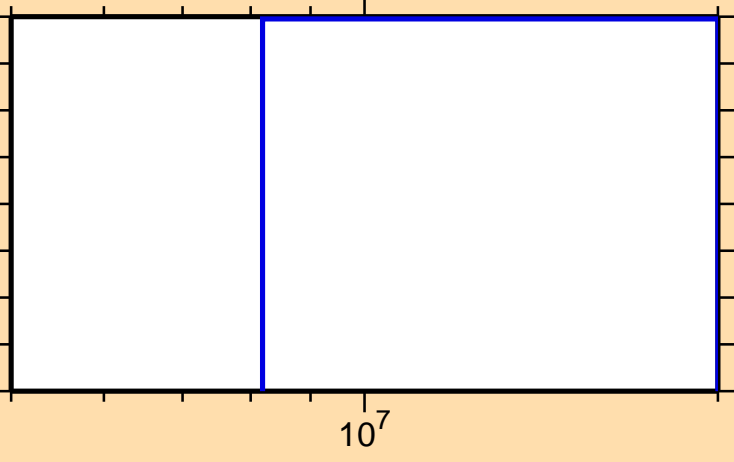
\sigma vs. E for ^{120}\text{In}(n,3n)
