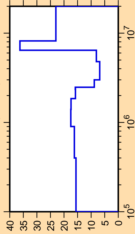
\Delta\sigma/\sigma vs. E for ^{120}\text{In}(n,\text{inel.})
