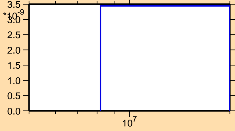
\sigma vs. E for ^{120}\text{In}(n,2np)
