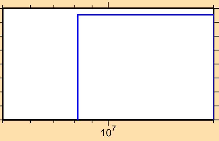
\sigma vs. E for ^{120}\text{In}(n,nd)
