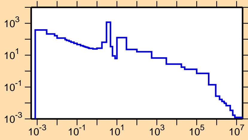
\sigma vs. E for ^{120}\text{In}(n,\gamma)
