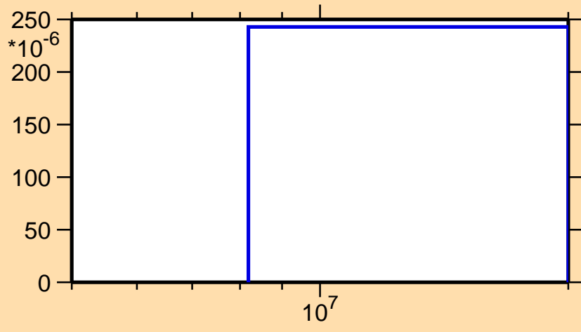
\sigma vs. E for ^{120}\text{In}(n,d)
