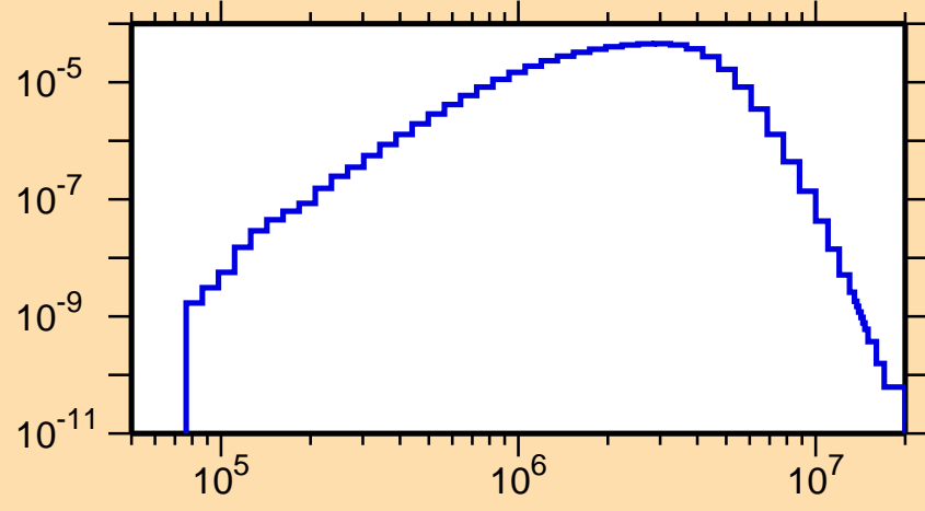
\sigma vs. E for ^{120}\text{In}(n,n_3)
