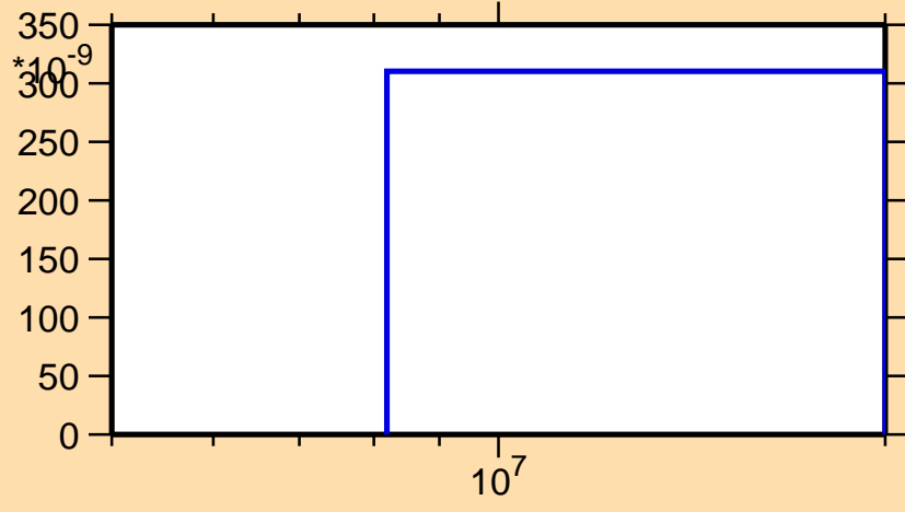
\sigma vs. E for ^{121}\text{In}(n,n\alpha)
