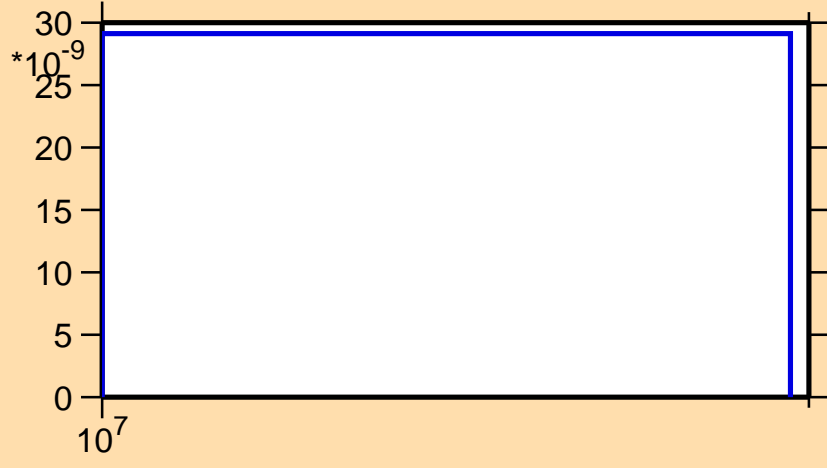
\sigma vs. E for ^{122}\text{In}(n,\text{nd})
