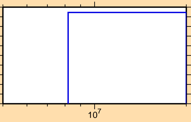
\sigma vs. E for ^{122}\text{In}(n,nd)
