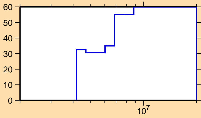
\Delta\sigma/\sigma vs. E for ^{122}\text{In}(n,n\text{cont.})
