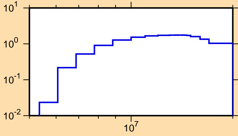
\sigma vs. E for ^{122}\text{In}(n,2n)
