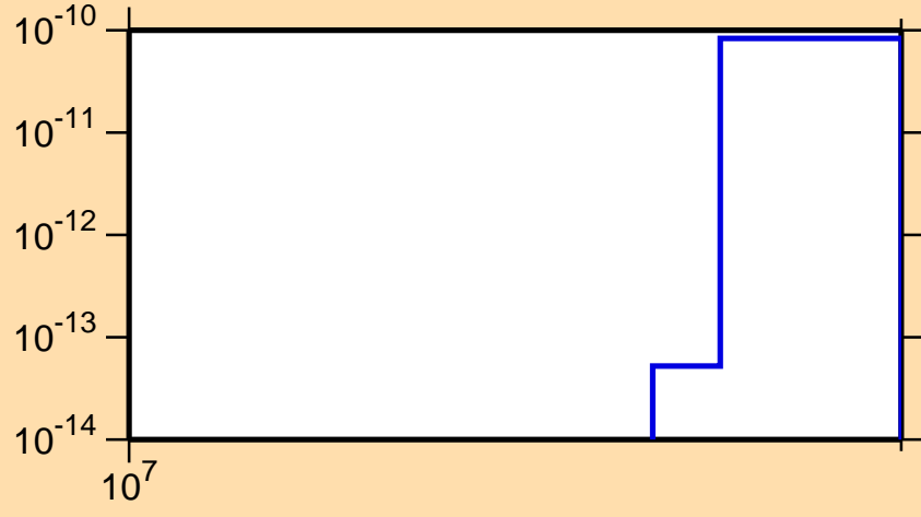
\sigma vs. E for ^{122}\text{In}(n,2n\alpha)
