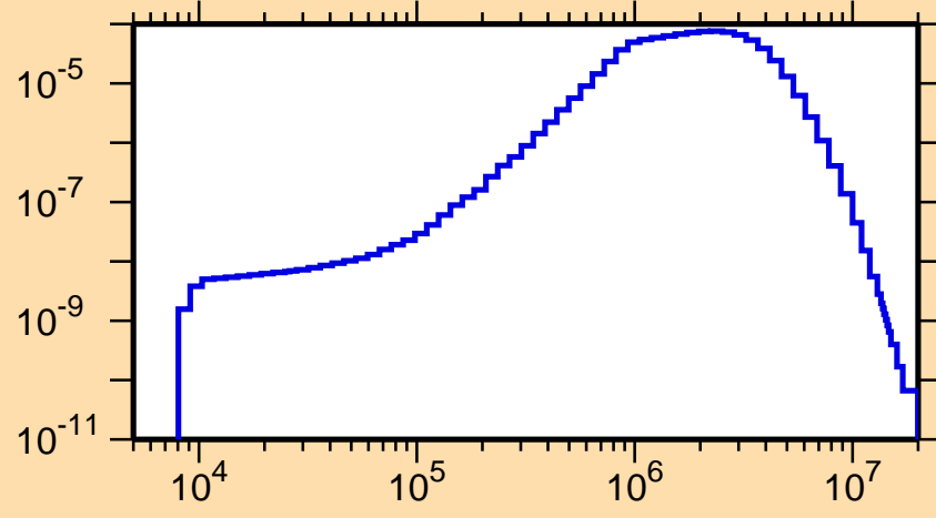
\sigma vs. E for ^{122}\text{In}(n,n_1)
