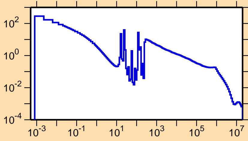
\sigma vs. E for ^{122}\text{In}(n,\gamma)
