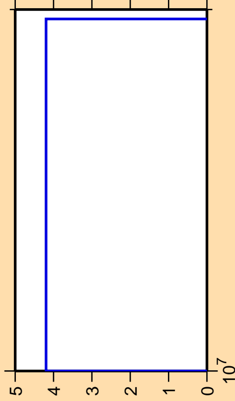
\Delta\sigma/\sigma vs. E for ^{122}\text{In}(n,2n\alpha)
