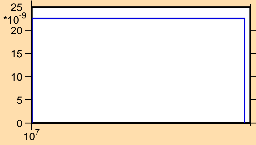
\sigma vs. E for ^{122}\text{In}(n,nd)
