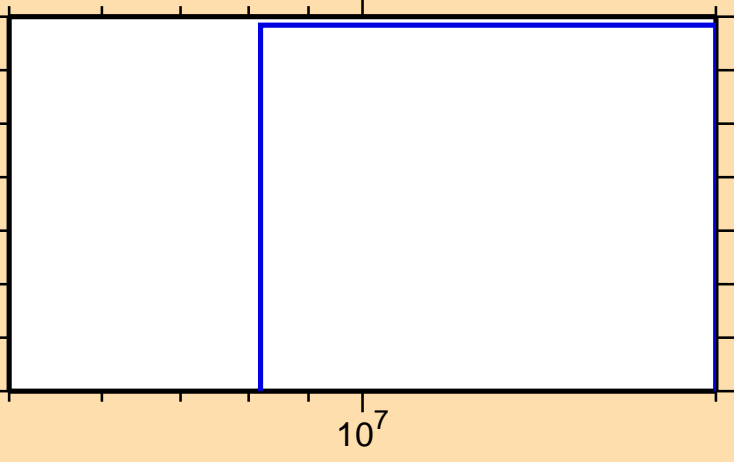
\sigma vs. E for ^{123}\text{In}(n,np)
