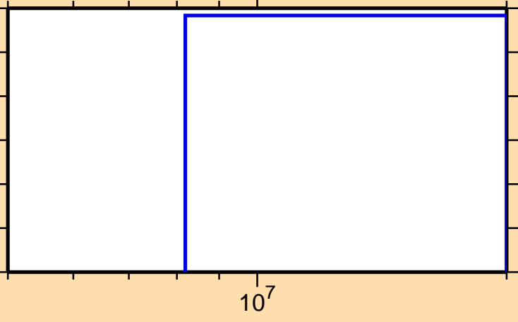
\sigma vs. E for ^{123}\text{In}(n,d)
