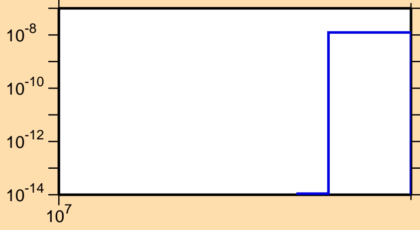
\sigma vs. E for ^{123}\text{In}(n,nd)
