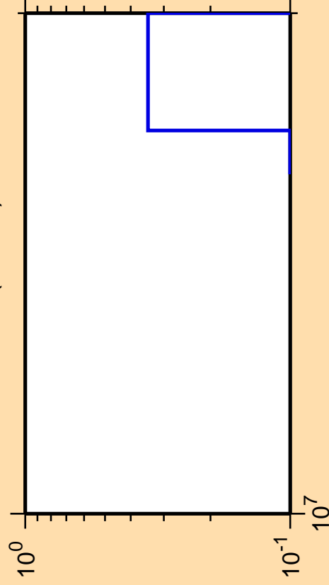
\Delta\sigma/\sigma vs. E for ^{123}\text{In}(n,2n\alpha)
