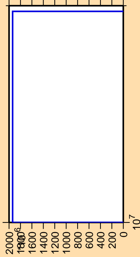
\Delta\sigma/\sigma vs. E for ^{123}\text{In}(n,2n\alpha)
