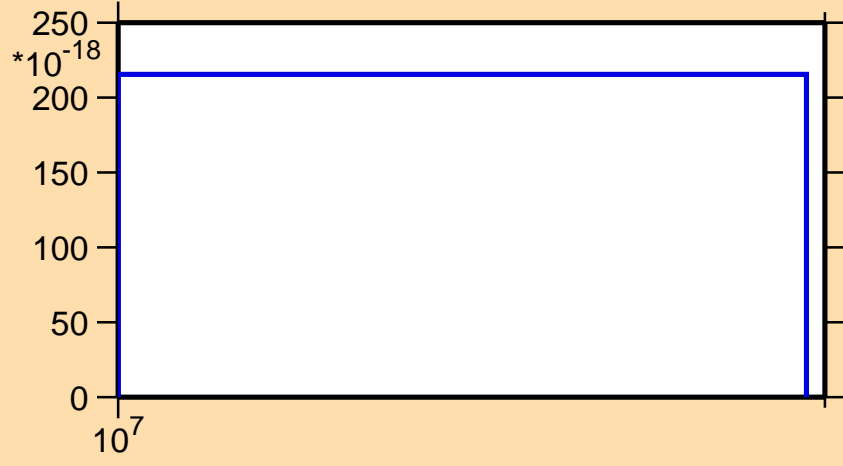
\sigma vs. E for ^{123}\text{In}(n,2n\alpha)
