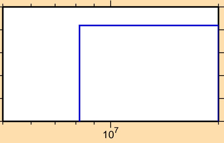
\sigma vs. E for ^{123}\text{In}(n,nt)
