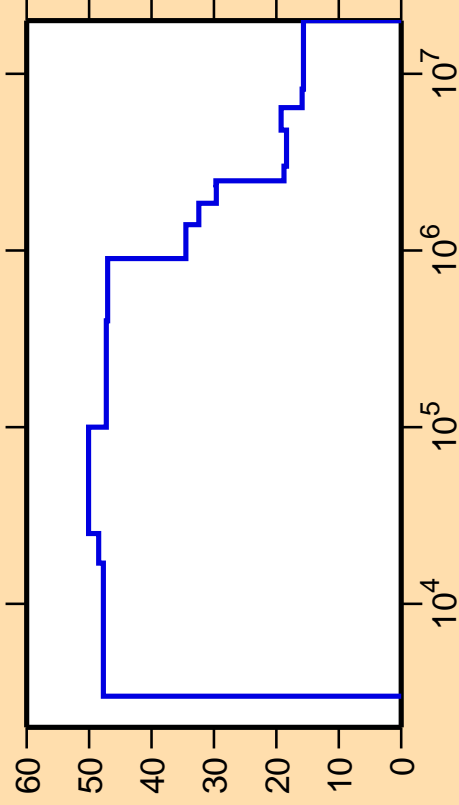
\Delta\sigma/\sigma vs. E for ^{123}\text{In}(n,\text{nonel.})
