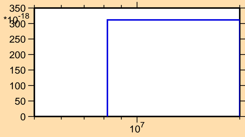
\sigma vs. E for ^{123}\text{In}(n,2n\alpha)
