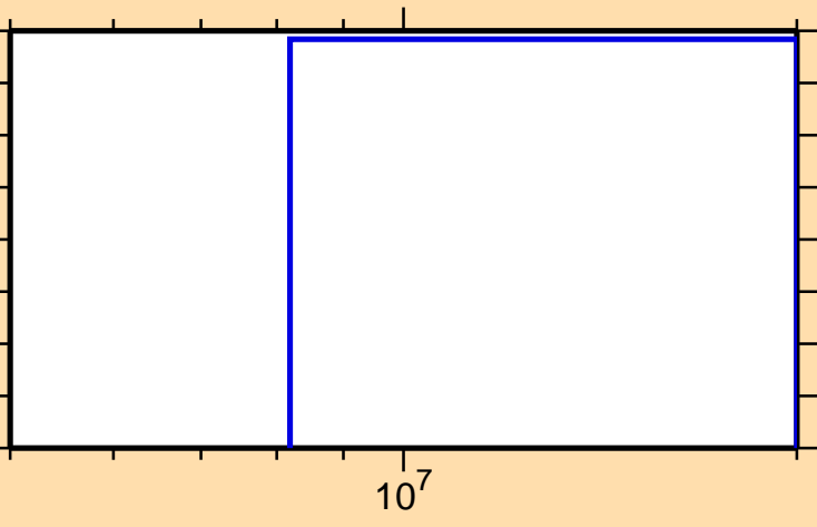
\sigma vs. E for ^{124}\text{In}(n,3n)
