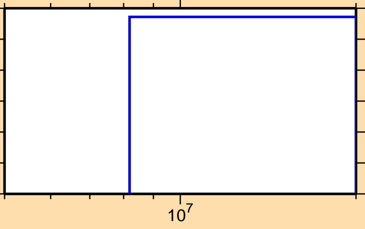
\sigma vs. E for ^{124}\text{In}(n,\text{nd})
