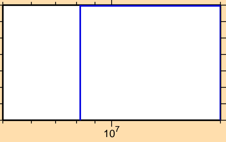
\sigma vs. E for ^{124}\text{In}(n,np)
