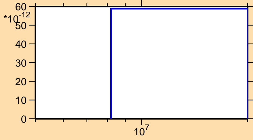
\sigma vs. E for ^{124}\text{In}(n,2np)
