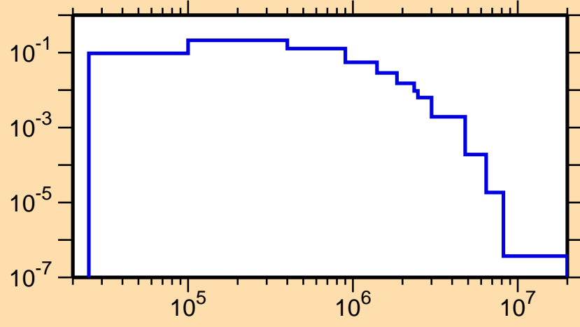
\sigma vs. E for ^{124}\text{In}(n,n_1)
