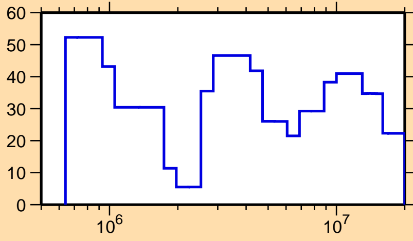
\Delta\sigma/\sigma vs. E for ^{124}\text{In}(n, el.)
