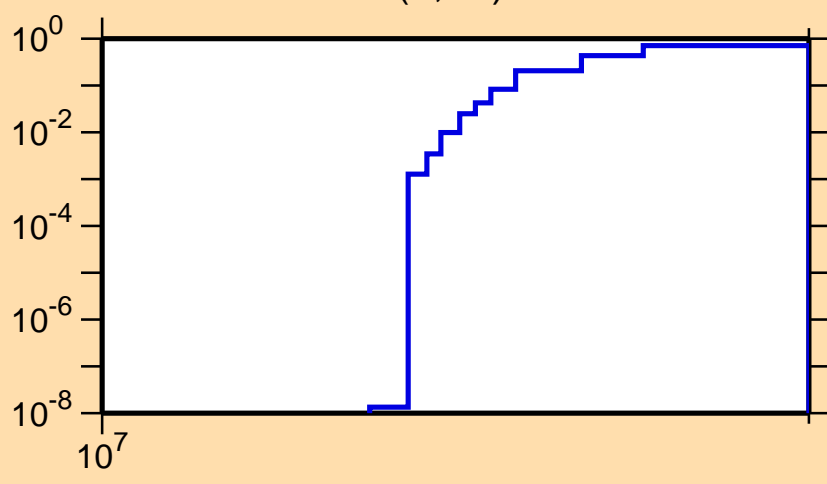
\sigma vs. E for ^{124}\text{In}(n,3n)
