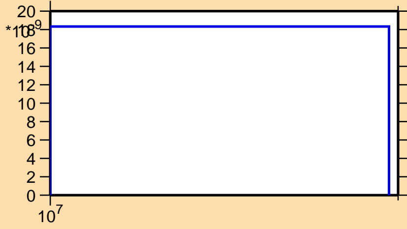
\sigma vs. E for ^{124}\text{In}(n,n\alpha)
