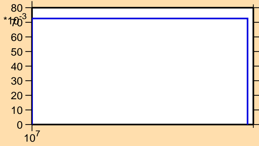
\sigma vs. E for ^{124}\text{In}(n,3n)
