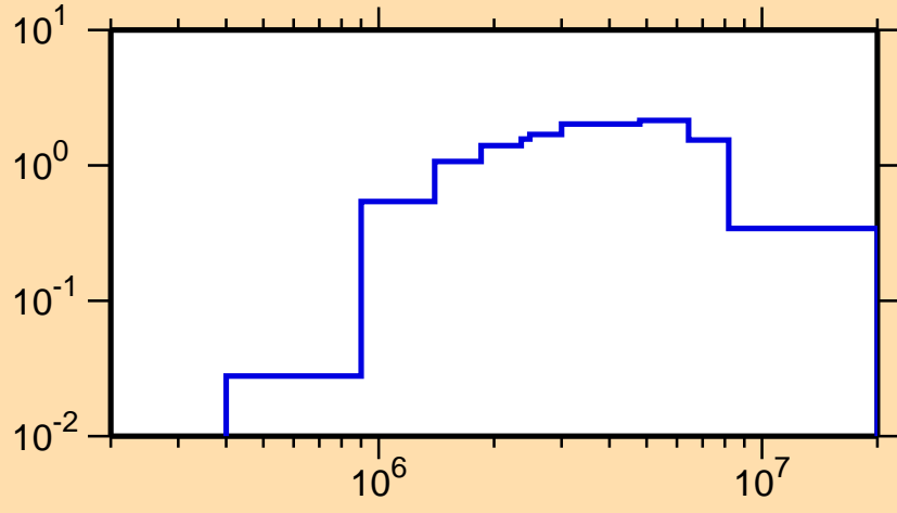
\sigma vs. E for ^{124}\text{In}(n,n\text{cont.})
