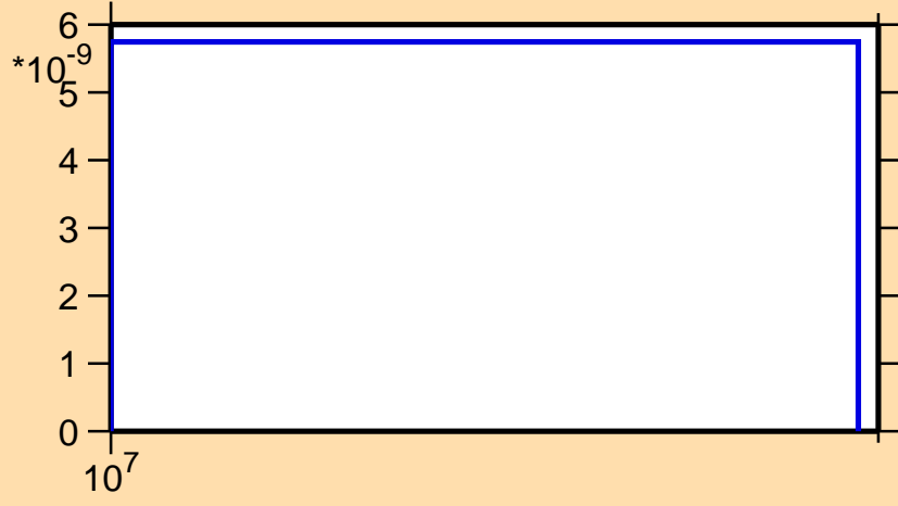
\sigma vs. E for ^{125}\text{In}(n,n\alpha)
