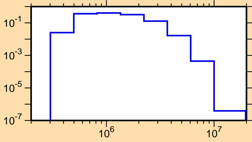
\sigma vs. E for ^{125}\text{In}(n,n_2)
