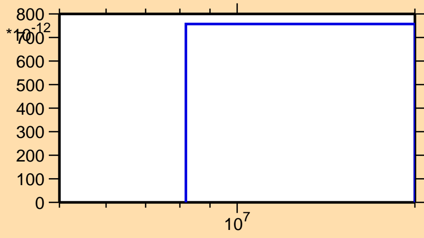
\sigma vs. E for ^{126}\text{In}(n,n\alpha)
