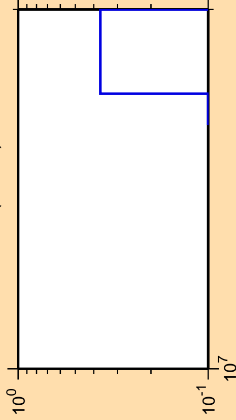
\Delta\sigma/\sigma vs. E for ^{126}\text{In}(n,2n\alpha)
