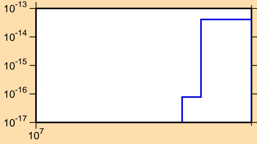
\sigma vs. E for ^{126}\text{In}(n,2n\alpha)
