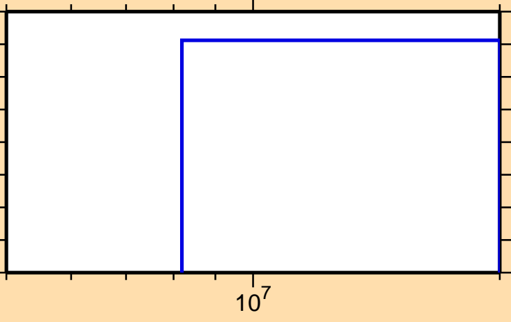
\sigma vs. E for ^{126}\text{In}(n,\alpha)
