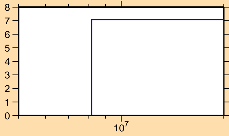
\Delta\sigma/\sigma vs. E for ^{126}\text{In}(n,\text{nonel.})
