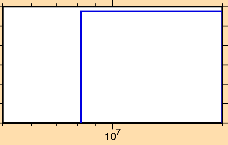
\sigma vs. E for ^{127}\text{In}(n,\alpha)
