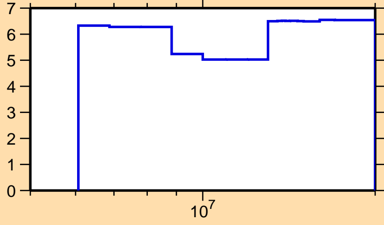
\Delta\sigma/\sigma vs. E for ^{127}\text{In}(n,\text{nonel.})
