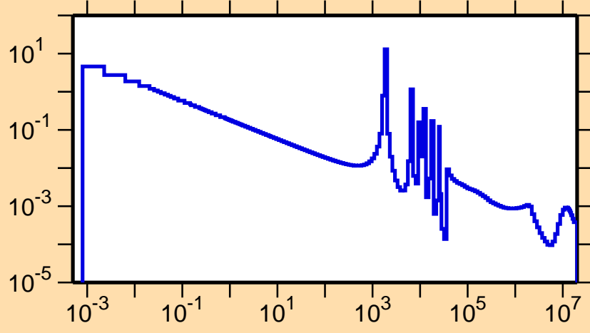
\sigma vs. E for ^{127}\text{In}(n,\gamma)
