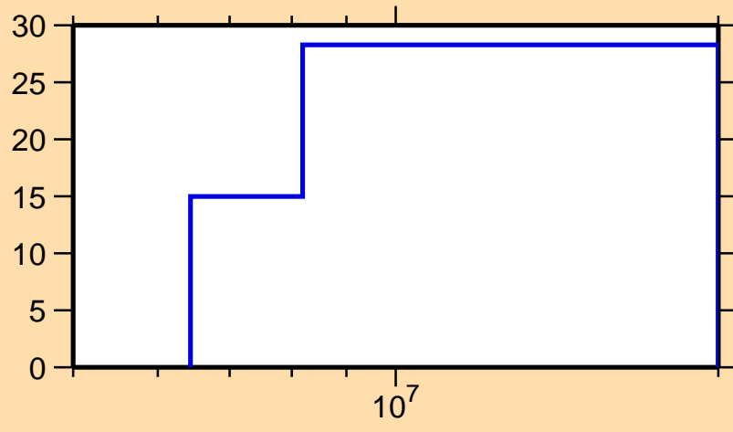
\Delta\sigma/\sigma vs. E for ^{127}\text{In}(n,ncont.)
