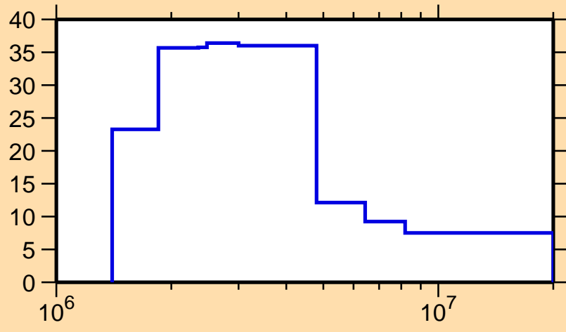
\Delta\sigma/\sigma vs. E for ^{127}\text{In}(n, el.)
