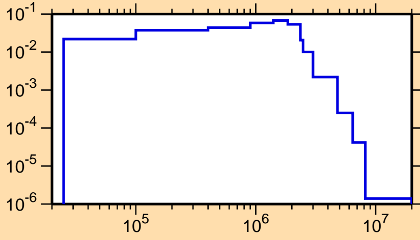
\sigma vs. E for ^{127}\text{In}(n,n_1)
