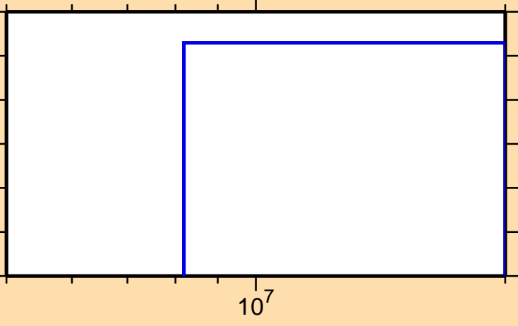
\sigma vs. E for ^{127}\text{In}(n,n\alpha)
