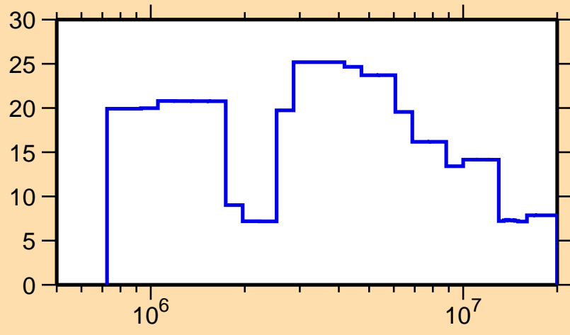
\Delta\sigma/\sigma vs. E for ^{171}\text{Ir}(n,el.)
