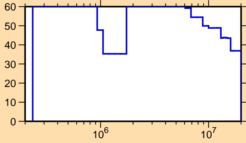
\Delta\sigma/\sigma vs. E for ^{171}\text{Ir}(n,n_1)
