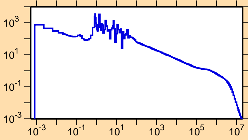
\sigma vs. E for ^{171}\text{Ir}(n,\gamma)
