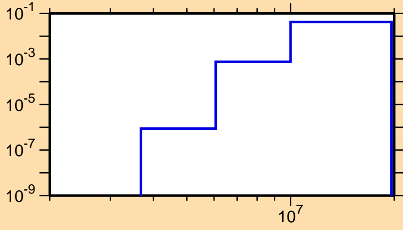
\sigma vs. E for ^{171}\text{Ir}(\text{mt } 45)
