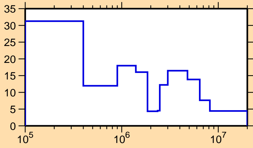
\Delta\sigma/\sigma vs. E for ^{171}\text{Ir}(n,\text{tot.})
