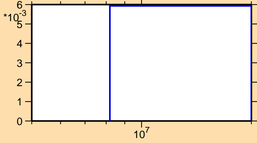
\sigma vs. E for ^{171}\text{Ir}(n,2n)
