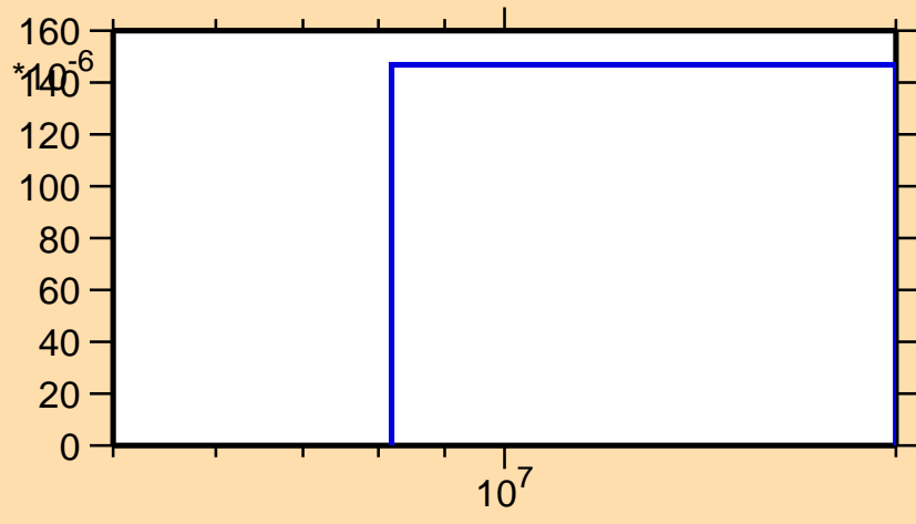
\sigma vs. E for ^{171}\text{Ir}(n,2np)
