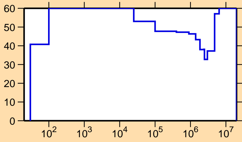
\Delta\sigma/\sigma vs. E for ^{171}\text{Ir}(n,p)
