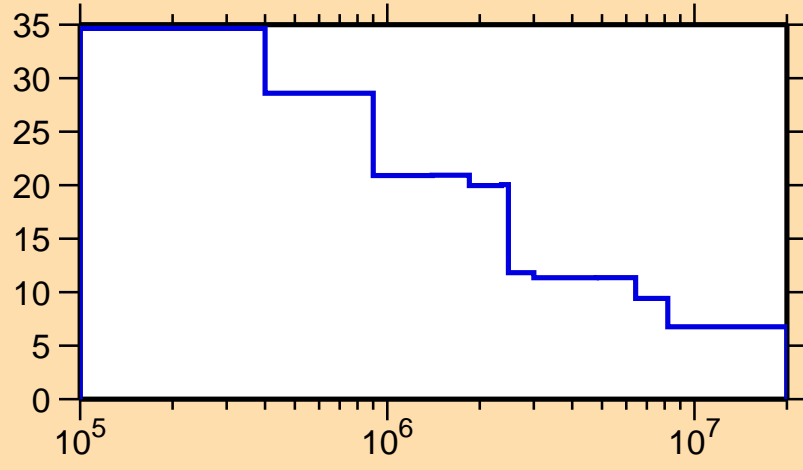
\Delta\sigma/\sigma vs. E for ^{171}\text{Ir}(n,\text{nonel.})
