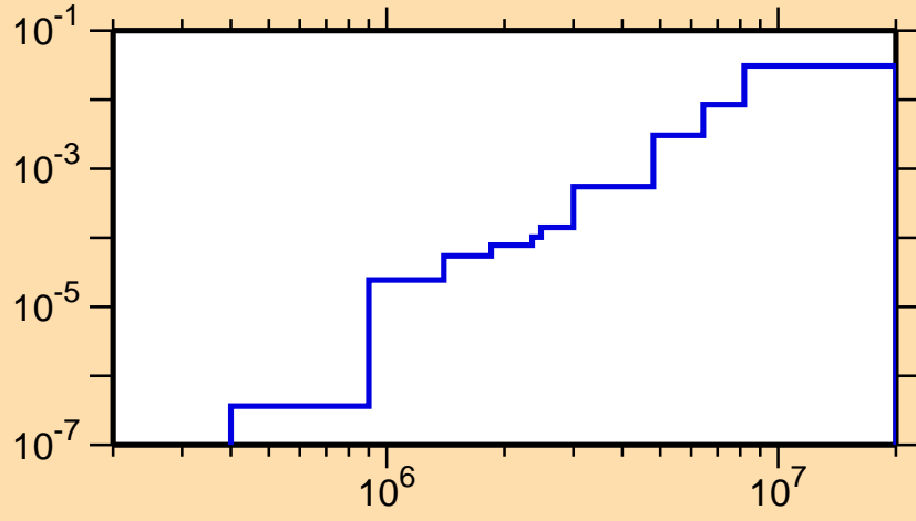
\sigma vs. E for ^{171}\text{Ir}(n,n\alpha)
