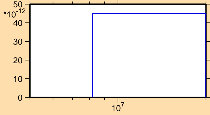
\sigma vs. E for ^{171}\text{Ir}(\text{mt } 34)
