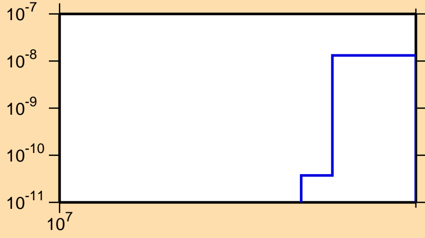
\sigma vs. E for ^{172}\text{Ir}(n,nt)
