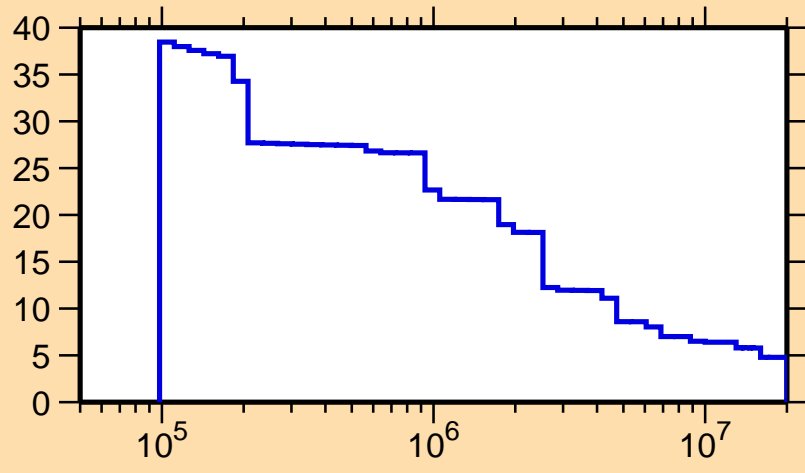
\Delta\sigma/\sigma vs. E for ^{172}\text{Ir}(n,\text{nonel.})
