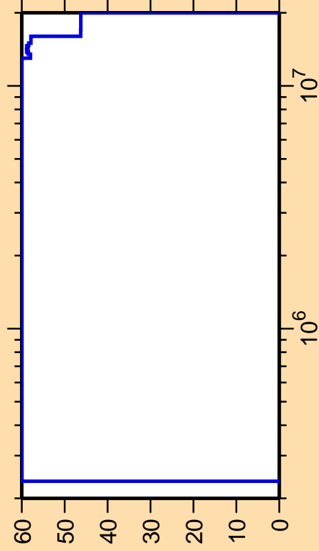
\Delta\sigma/\sigma vs. E for ^{172}\text{Ir}(n,n\text{cont.})
