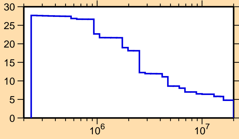
\Delta\sigma/\sigma vs. E for ^{172}\text{Ir}(n,n\text{onel.})
