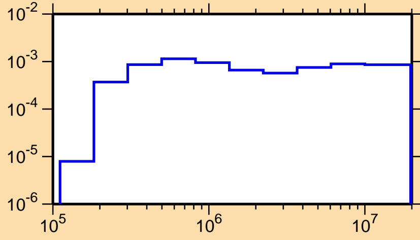
\sigma vs. E for ^{172}\text{Ir}(n,n_3)
