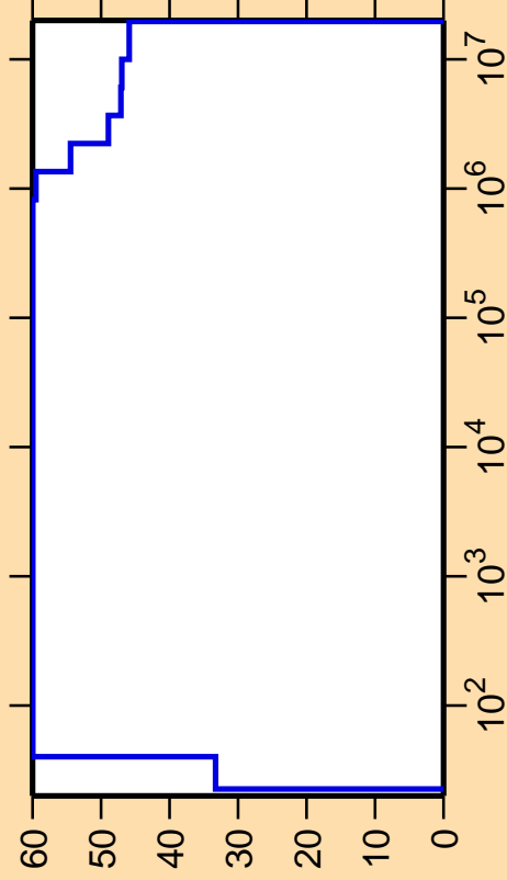
\Delta\sigma/\sigma vs. E for ^{172}\text{Ir}(n,p)
