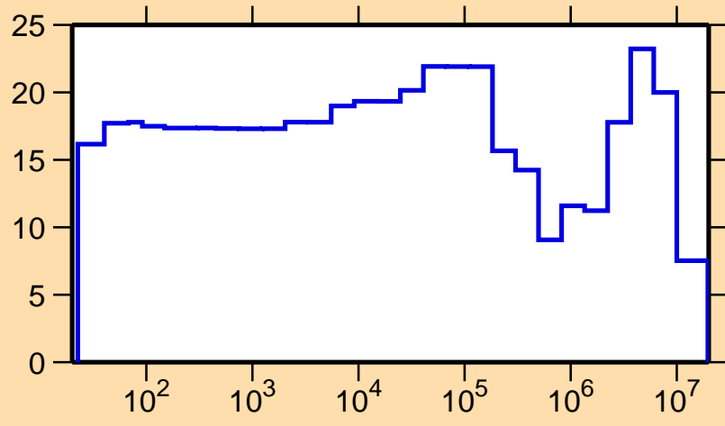
\Delta\sigma/\sigma vs. E for ^{172}\text{Ir}(n,el.)
