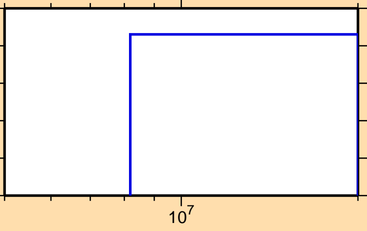
\sigma vs. E for ^{172}\text{Ir}(n,\text{nd})
