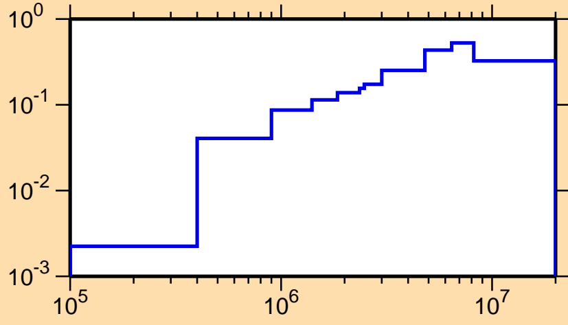
\sigma vs. E for ^{172}\text{Ir}(n,n\text{cont.})
