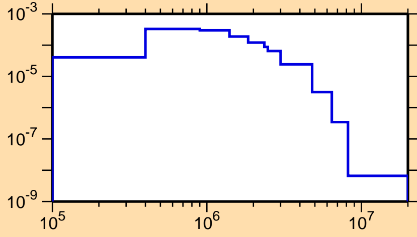
\sigma vs. E for ^{172}\text{Ir}(n,n_2)
