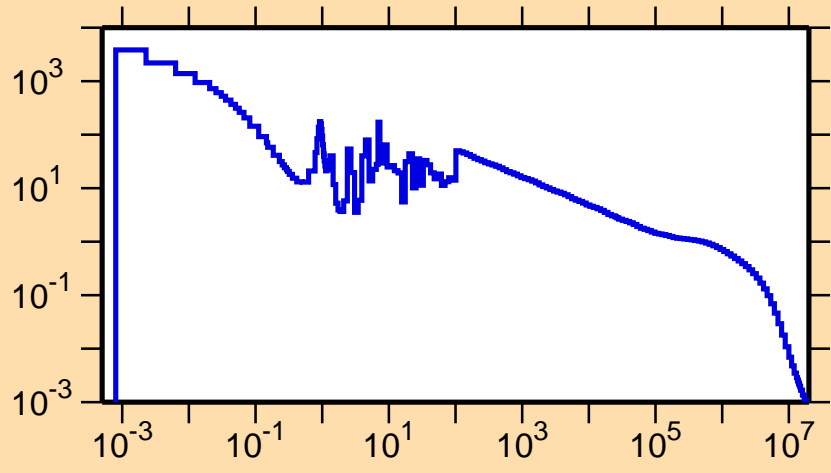
\sigma vs. E for ^{172}\text{Ir}(n,\gamma)
