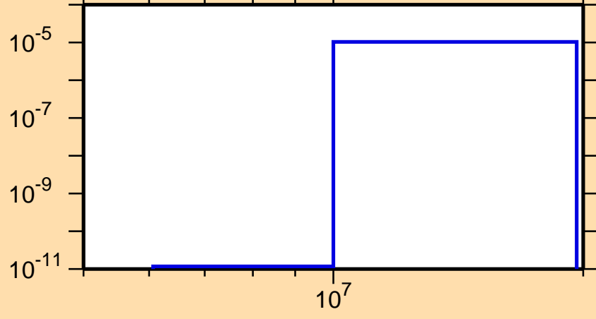
\sigma vs. E for ^{172}\text{Ir}(n,\text{pd})
