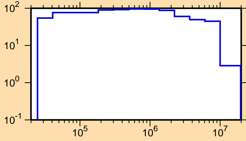
\Delta\sigma/\sigma vs. E for ^{172}\text{Ir}(n,n_1)
