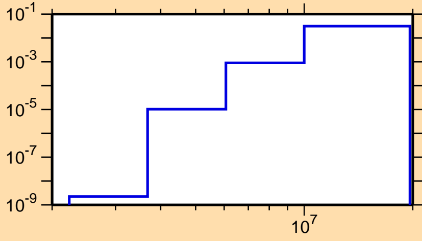
\sigma vs. E for ^{172}\text{Ir}(\text{mt } 45)
