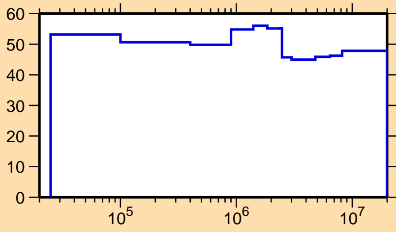
\Delta\sigma/\sigma vs. E for ^{172}\text{Ir}(n,n\text{cont.})
