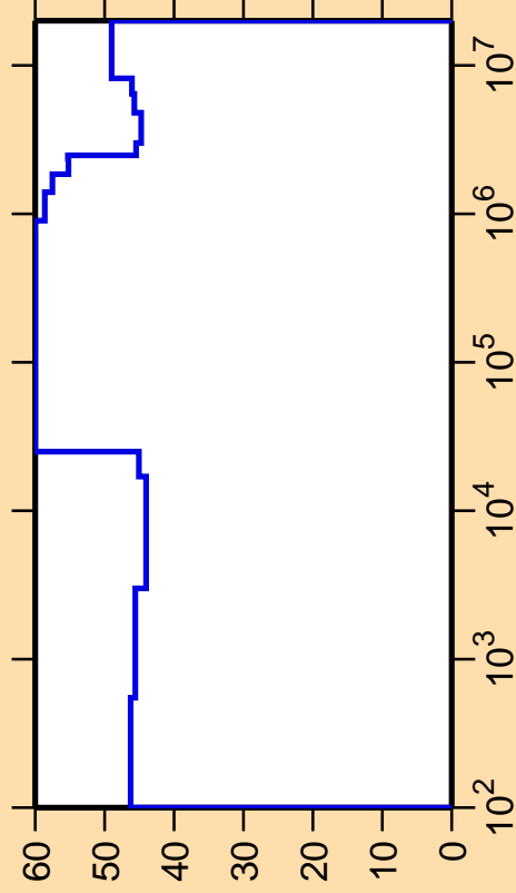
\Delta\sigma/\sigma vs. E for ^{172}\text{Ir}(n,\text{inel.})
