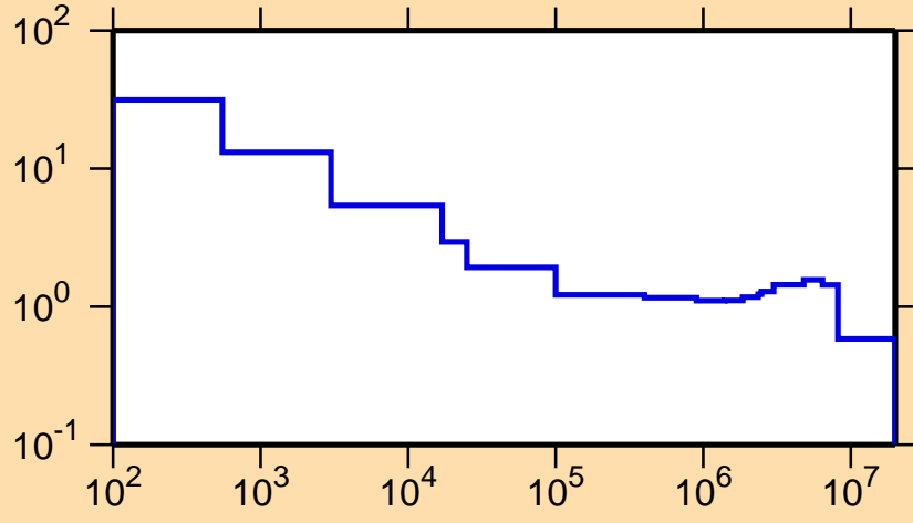
\sigma vs. E for ^{172}\text{Ir}(n,p)
