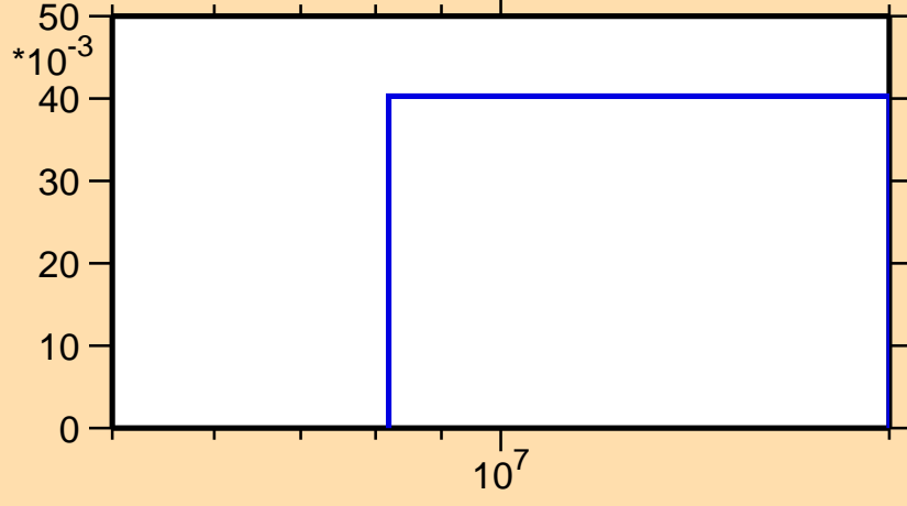
\sigma vs. E for ^{172}\text{Ir}(n,2n)
