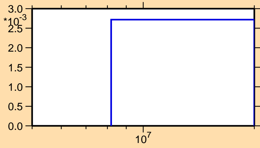
\sigma vs. E for ^{172}\text{Ir}(n,2np)
