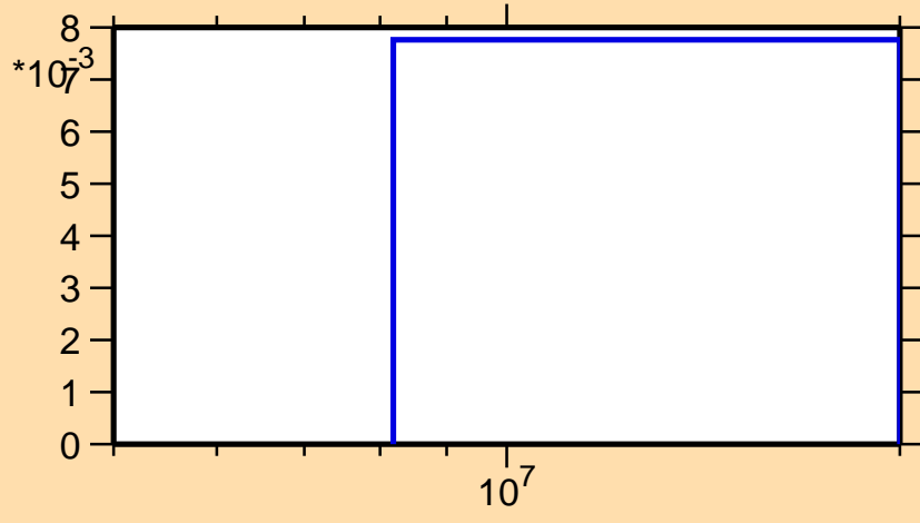
\sigma vs. E for ^{172}\text{Ir}(n,2n\alpha)
