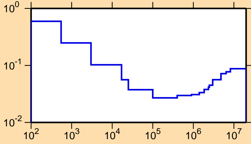
\sigma vs. E for ^{172}\text{Ir}(n,p\alpha)
