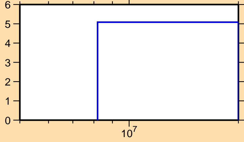
\Delta\sigma/\sigma vs. E for ^{172}\text{Ir}(n,\text{el.})
