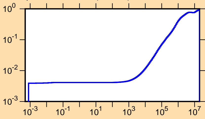
\mu vs. E for ^{173}\text{Ir}(\text{mt251})
