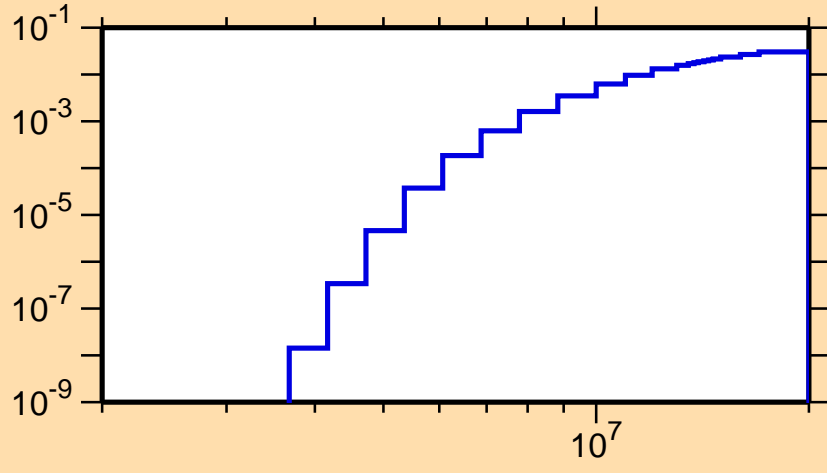
\sigma vs. E for ^{173}\text{Ir}(mt\ 45)
