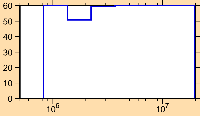
\Delta\sigma/\sigma vs. E for ^{173}\text{Ir}(n, el.)
