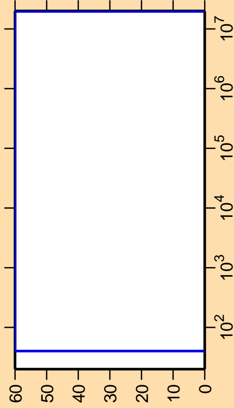
\Delta\sigma/\sigma vs. E for ^{173}\text{Ir}(n,\alpha)
