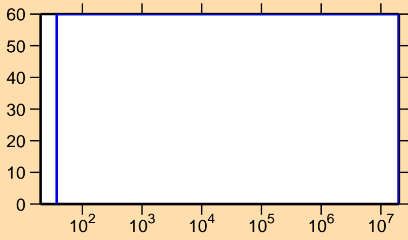
\Delta\sigma/\sigma vs. E for ^{174}\text{Ir}(n,\gamma)
