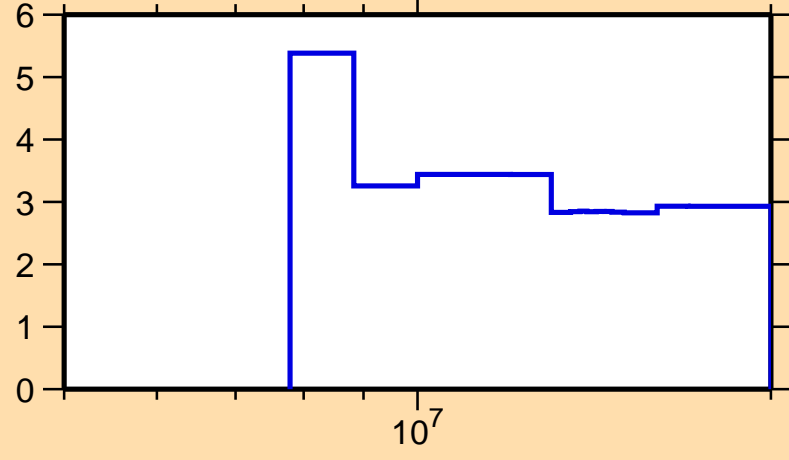
\Delta\sigma/\sigma vs. E for ^{174}\text{Ir}(n,\text{tot.})
