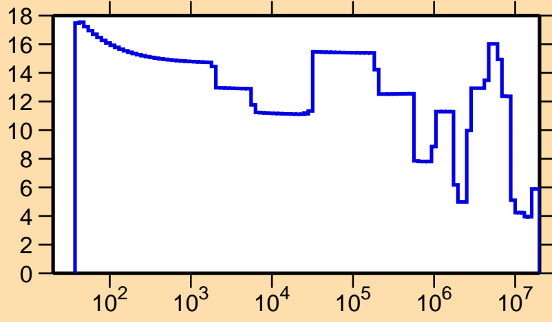
\Delta\sigma/\sigma vs. E for ^{174}\text{Ir}(n,el.)
