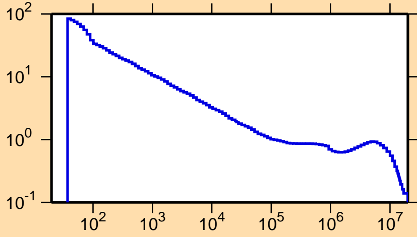
\sigma vs. E for ^{174}\text{Ir}(n,p)
