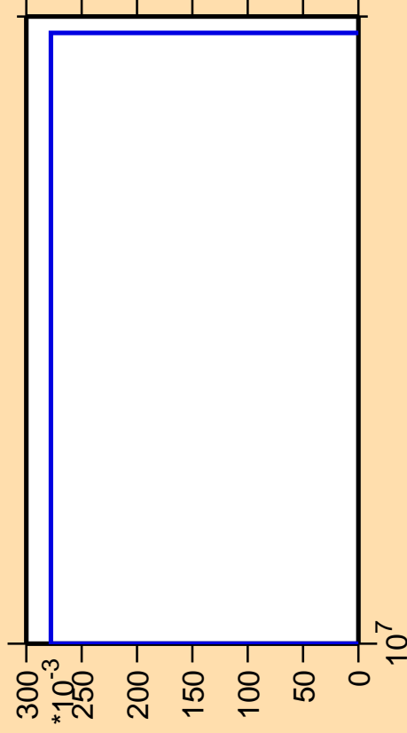
\Delta\sigma/\sigma vs. E for ^{174}\text{Ir}(n,3n\alpha)
