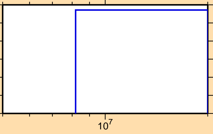
\sigma vs. E for ^{174}\text{Ir}(n,\text{nd})
