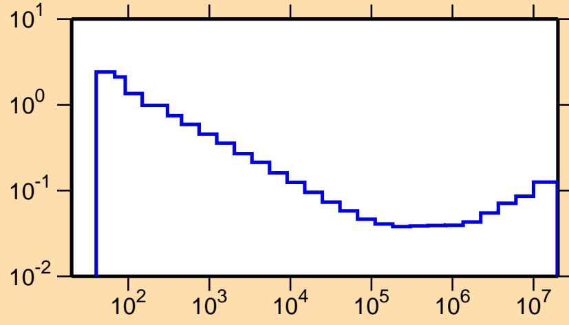
\sigma vs. E for ^{174}\text{Ir}(n,\alpha)
