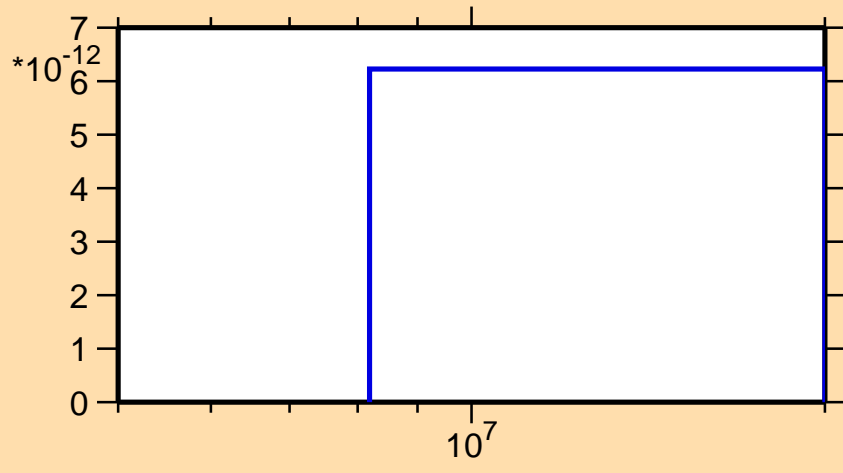
\sigma vs. E for ^{174}\text{Ir}(n,3n\alpha)
