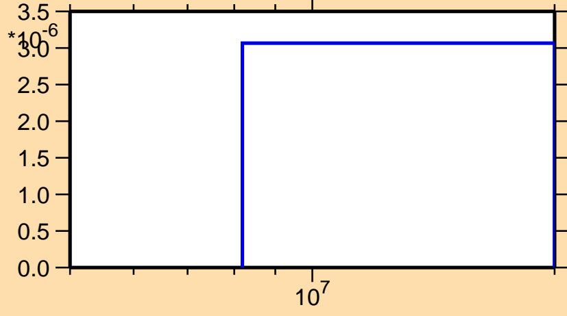
\sigma vs. E for ^{174}\text{Ir}(n,\text{nd})
