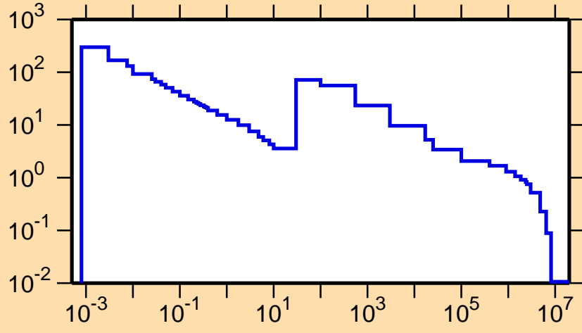
\sigma vs. E for ^{174}\text{Ir}(n,\gamma)
