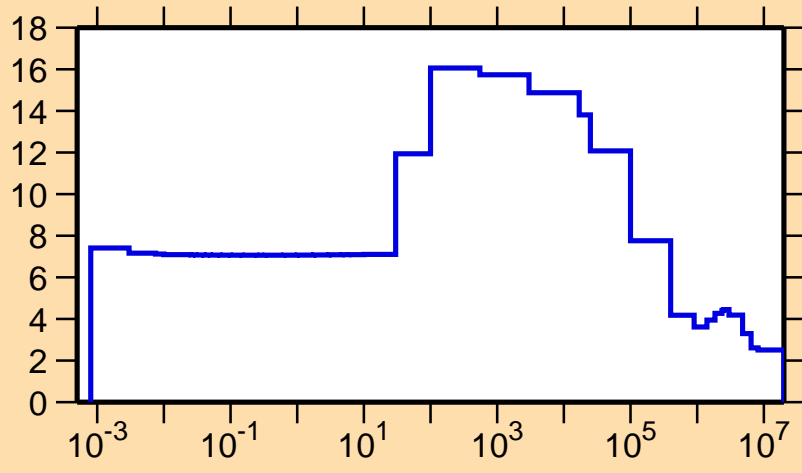
\sigma vs. E for ^{174}\text{Ir}(n,\text{el.})
