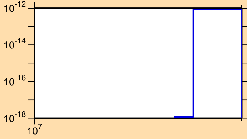
\sigma vs. E for ^{175}\text{Ir}(n,3n\alpha)
