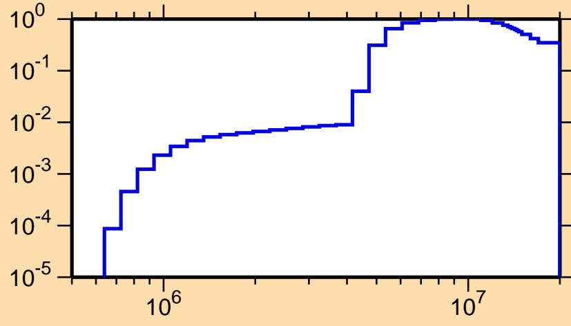
\sigma vs. E for ^{175}\text{Ir}(n,n\text{cont.})
