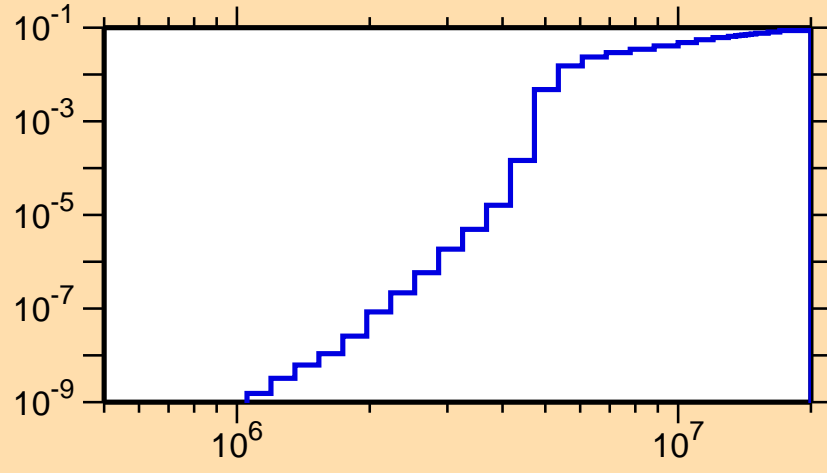
\sigma vs. E for ^{175}\text{Ir}(n,n\alpha)
