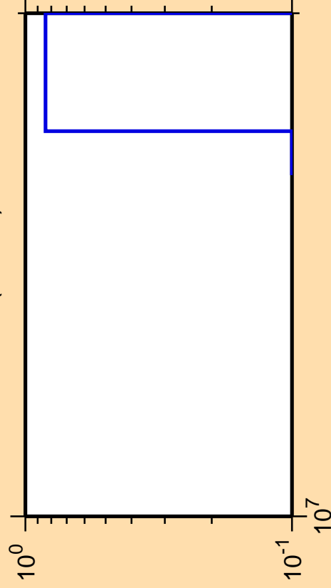
\Delta\sigma/\sigma vs. E for ^{175}\text{Ir}(n,3n\alpha)
