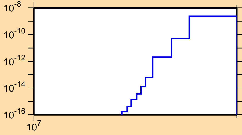
\sigma vs. E for ^{177}\text{Ir}(n,pt)
