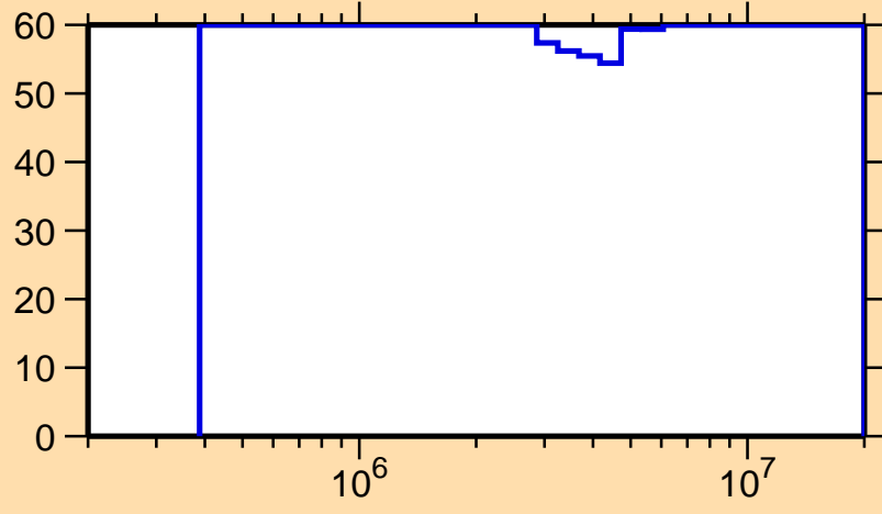
\Delta\sigma/\sigma vs. E for ^{177}\text{Ir}(n,n\text{cont.})
