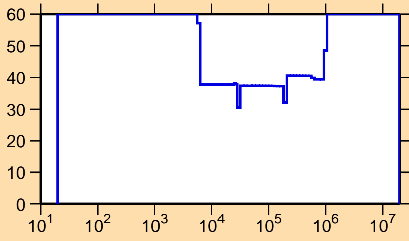
\Delta\sigma/\sigma vs. E for ^{177}\text{Ir}(n,\gamma)
