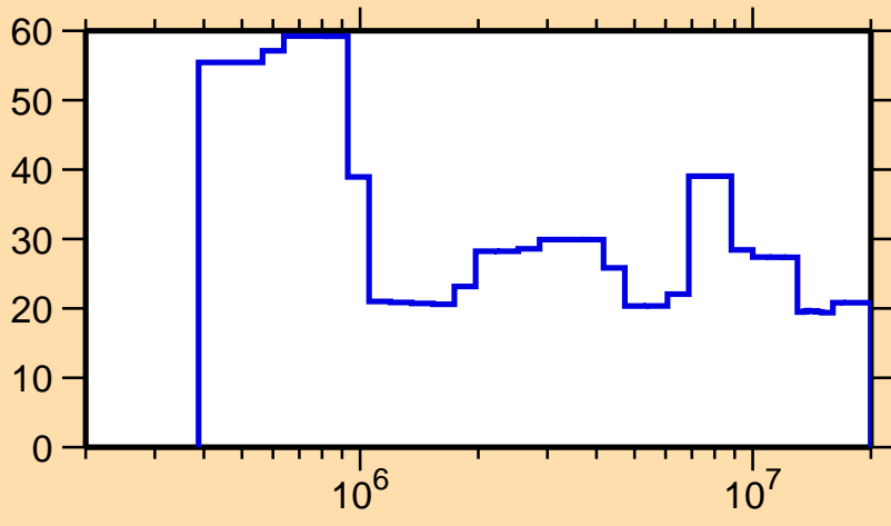
\Delta\sigma/\sigma vs. E for ^{177}\text{Ir}(n, el.)
