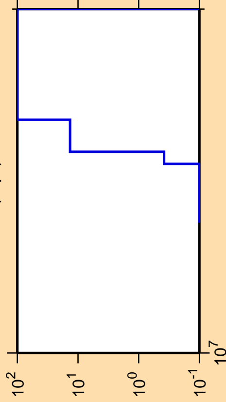
\Delta\sigma/\sigma vs. E for ^{177}\text{Ir}(n,pt)
