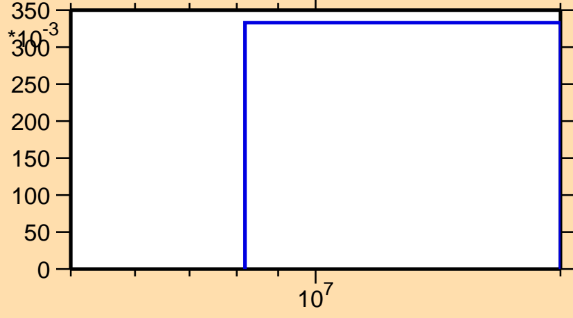
\sigma vs. E for ^{177}\text{Ir}(n,2n)
