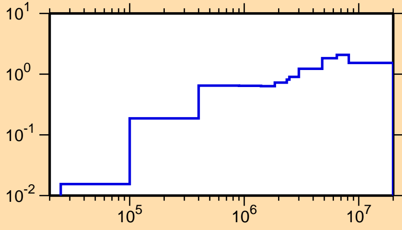
\sigma vs. E for ^{177}\text{Ir}(n,\text{inel.})
