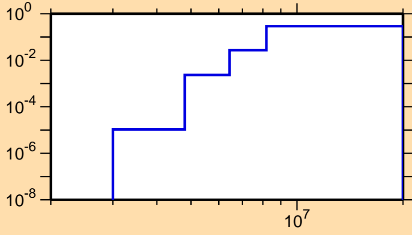
\sigma vs. E for ^{177}\text{Ir}(n,np)
