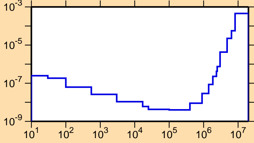
\sigma vs. E for ^{177}\text{Ir}(n,p\alpha)
