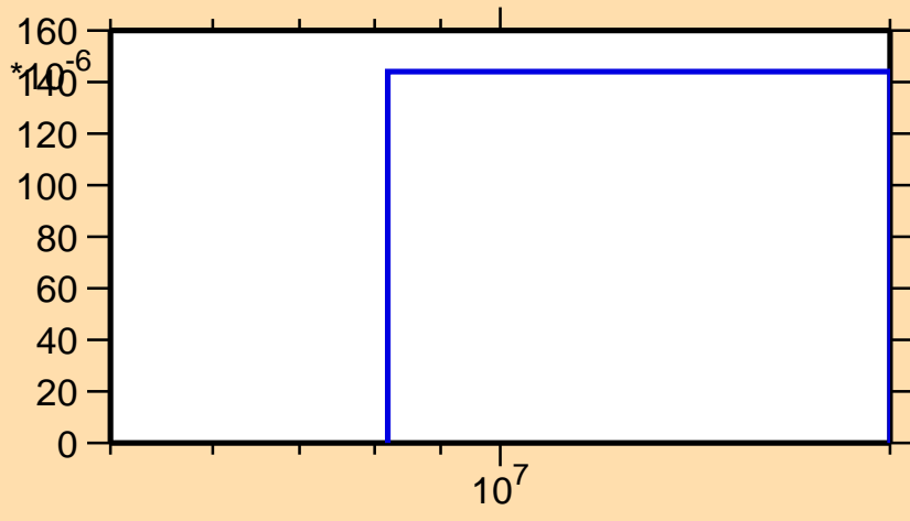
\sigma vs. E for ^{177}\text{Ir}(n,2np)
