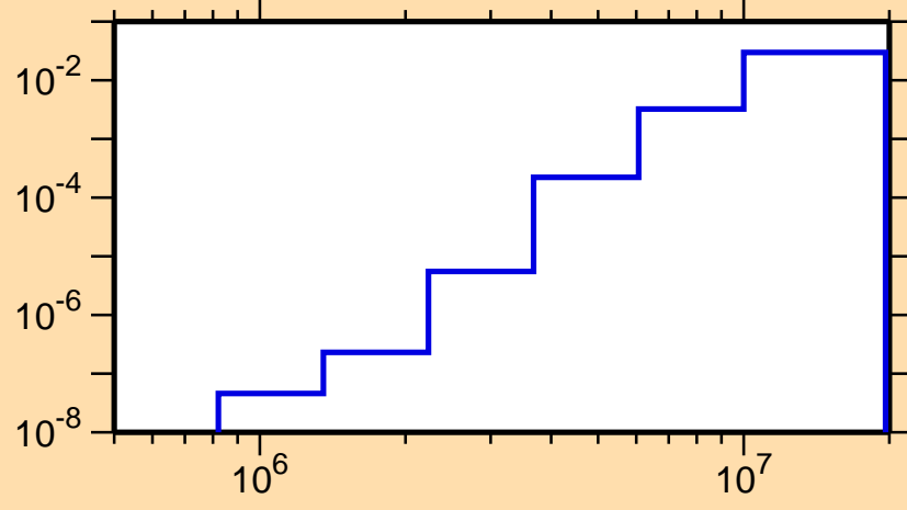
\sigma vs. E for ^{178}\text{Ir}(n,n\alpha)
