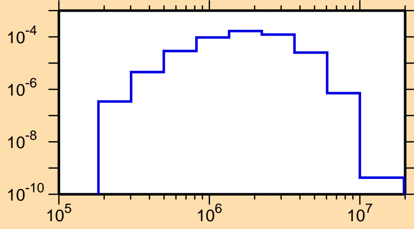
\sigma vs. E for ^{178}\text{Ir}(n,n_4)
