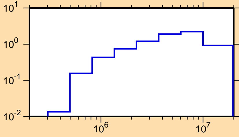
\sigma vs. E for ^{178}\text{Ir}(n,n\text{cont.})
