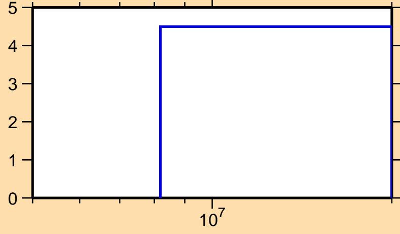
\Delta\sigma/\sigma vs. E for ^{178}\text{Ir}(n,\text{el.})
