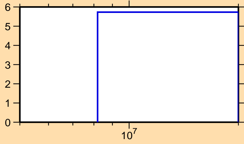
\Delta\sigma/\sigma vs. E for ^{178}\text{Ir}(n,\text{tot.})
