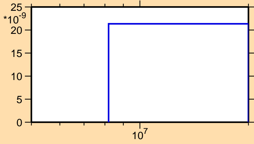
\sigma vs. E for ^{178}\text{Ir}(n,3n\alpha)
