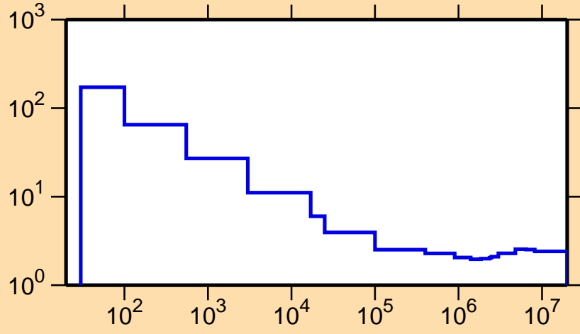
\sigma vs. E for ^{178}\text{Ir}(n,\text{nonel.})
