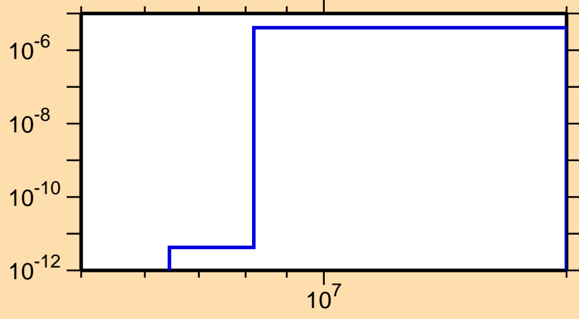
\sigma vs. E for ^{178}\text{Ir}(n,\text{He}3)
