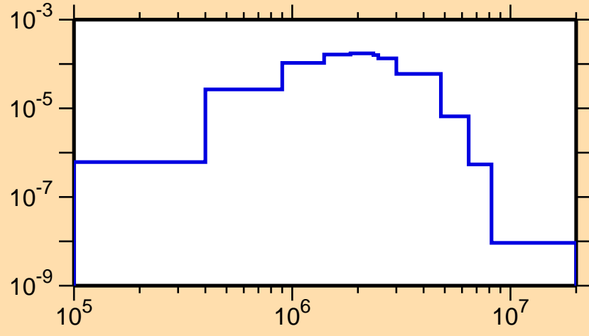
\sigma vs. E for ^{178}\text{Ir}(n,n_4)
